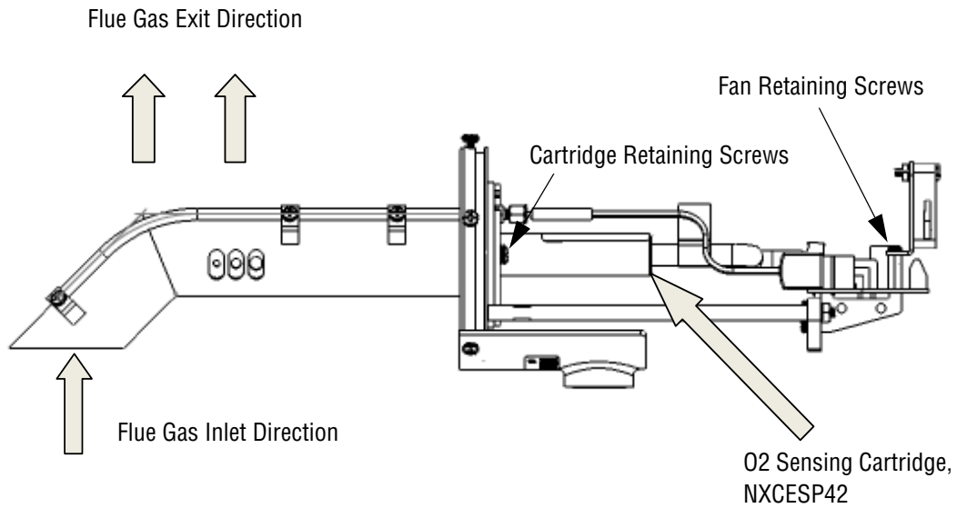
FIGURE 5. Flue Gas Flow through Probe
