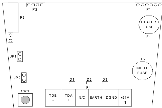
FIGURE 1. NXCES02 INTERNAL PC BOARD
