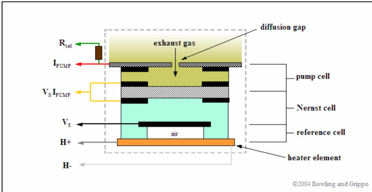
FIGURE 3. Wideband O 2 sensor - Internal structure
