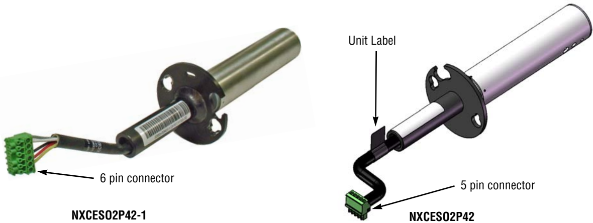
FIGURE 6. NXCESO2P42 Replacement Cartridges
