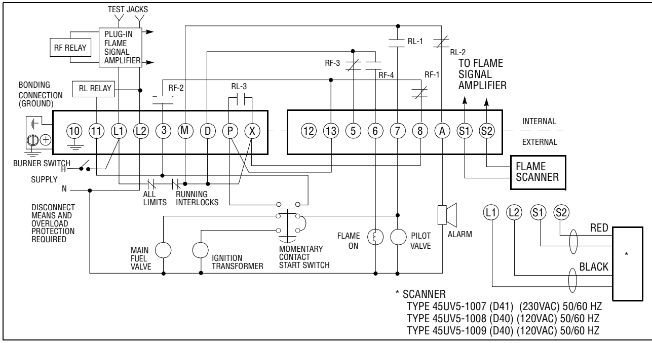
FIGURE 3. TYPICAL SCHEMATIC DIAGRAM FOR SEMI-AUTOMATIC PILOT IGNITED GAS OR OIL BURNER WITH PREPURGE, PILOT TFI, MAIN FLAME TFI AND INTERRUPTED PILOT
