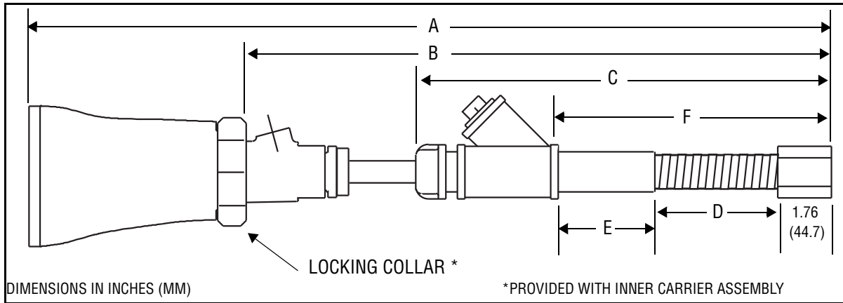
FIGURE 1. DIMENSIONS - SCANNER WITH FIBER OPTIC INNER AND OUTER CARRIERS
